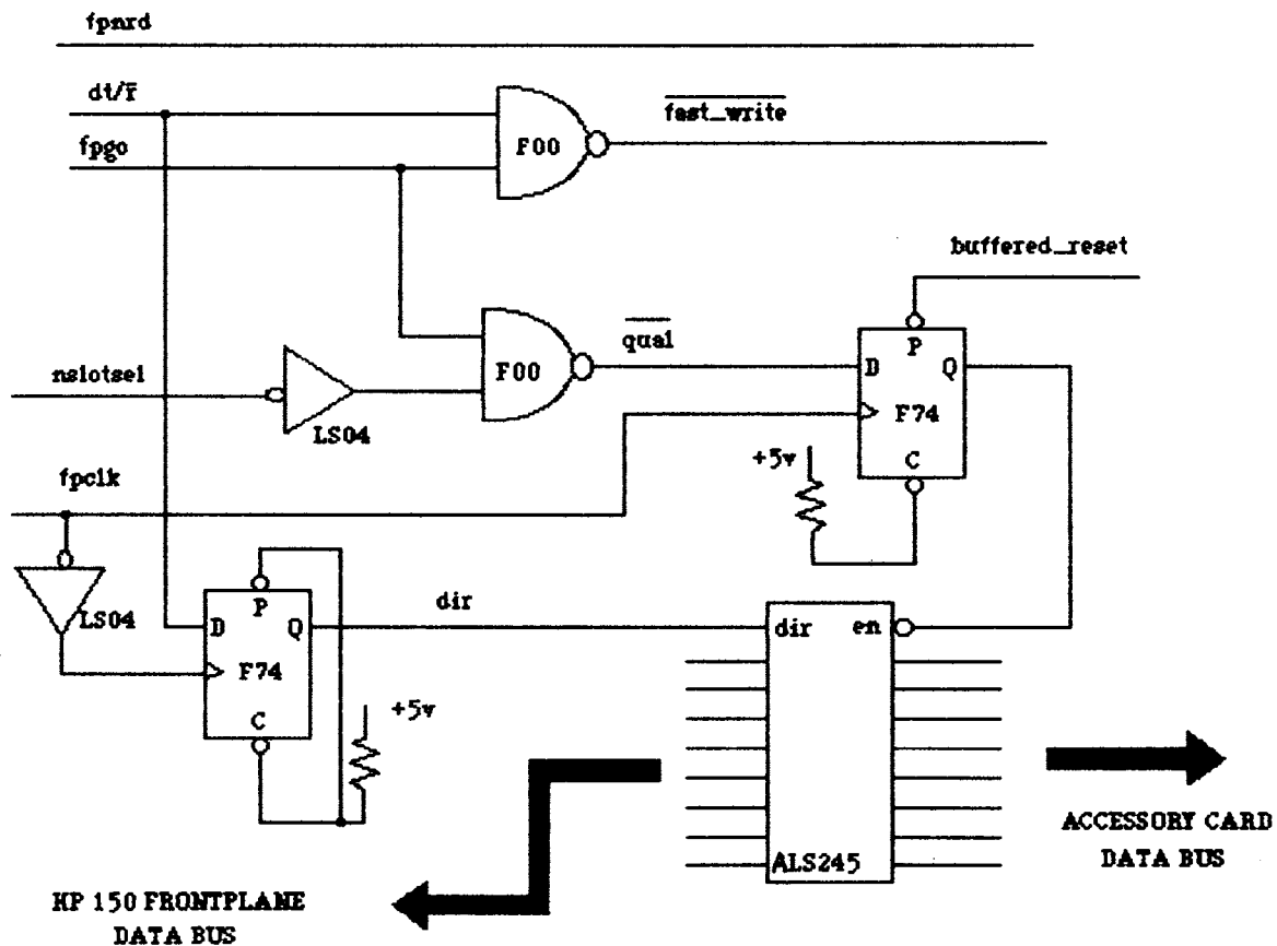
Figure 3-22. Tranceiver Schematic
