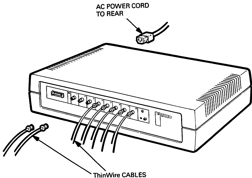
Figure 3-11: ThinWire Cables Connected to the DEMPR
