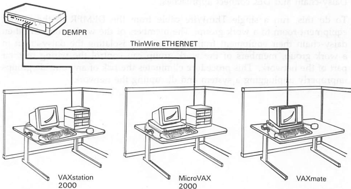
Figure 2-8: DECconnect Method of Wiring
