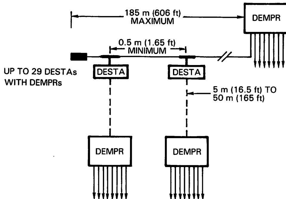
Figure 2-16: Stand-alone Cascading DEMPRs
