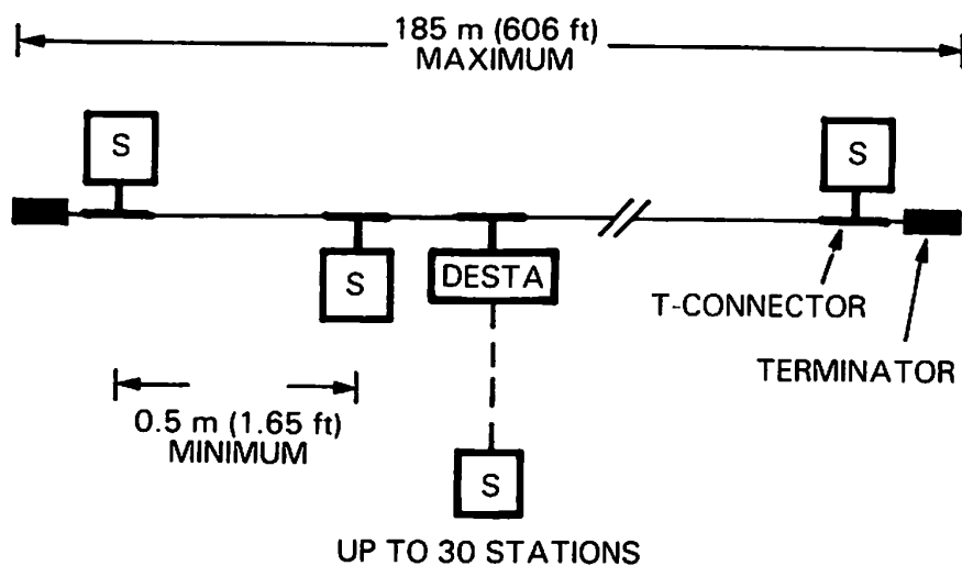
Figure 2-13: Single Segment ThinWire Configuration
