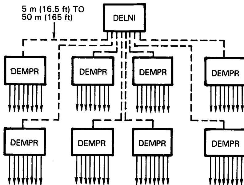
Figure 2-17: Stand-alone DELNI with DEMPRs
