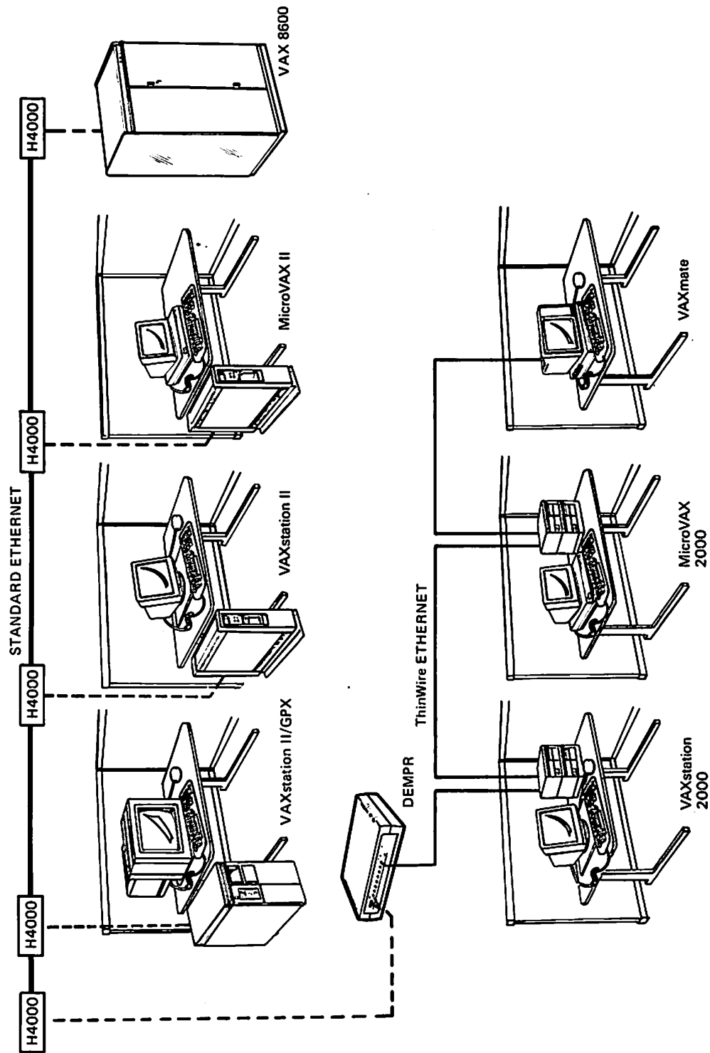
Figure 2-10: Connecting ThinWire Ethernet to Standard Ethernet
