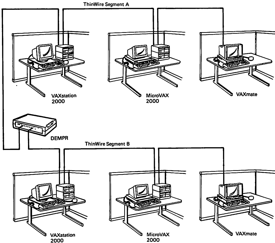
Figure 2-11: Multisegment ThinWire Configuration
