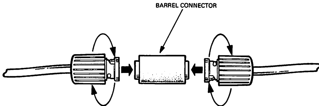
Figure 3-14: Connecting Two ThinWire Sections
