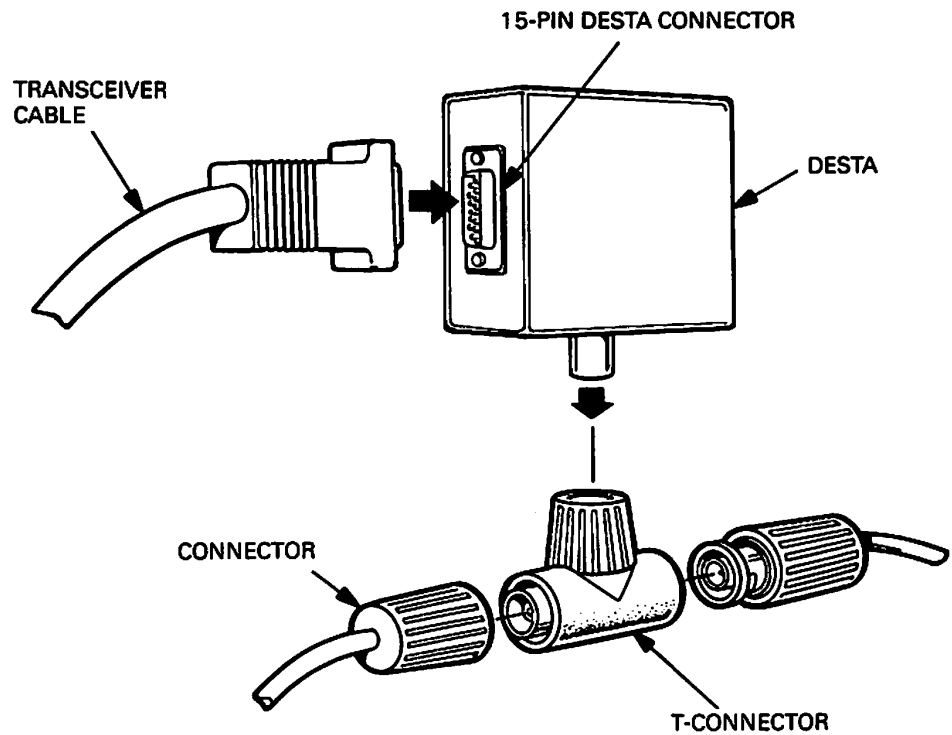
Figure 3–10: Attaching the Transceiver Cable to the DESTA
