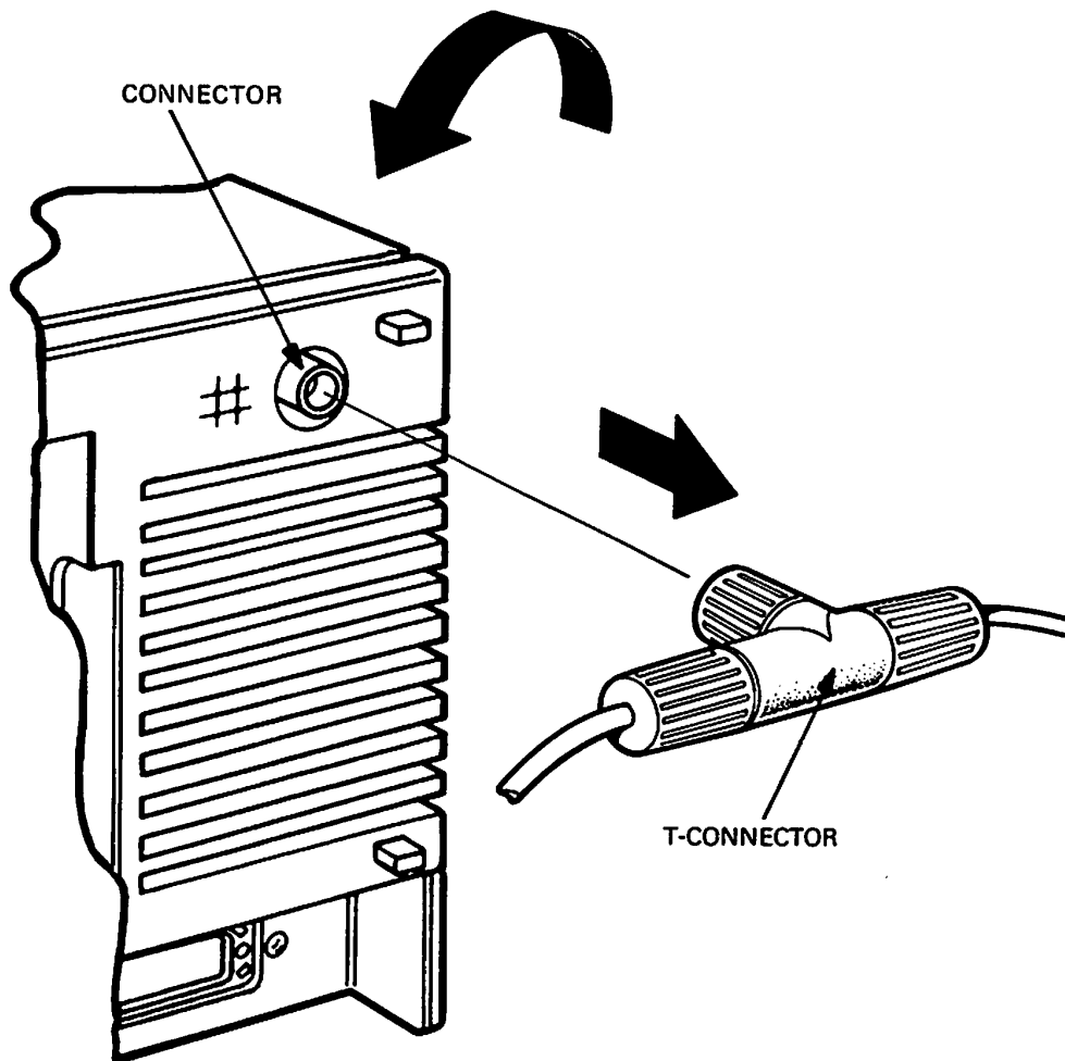
Figure 2-19: Disconnecting a Station from ThinWire Ethernet
