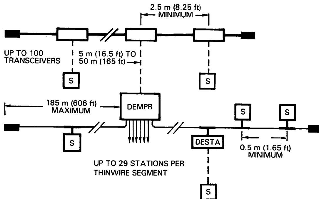
Figure 2-15: DEMPR on Standard Ethernet
