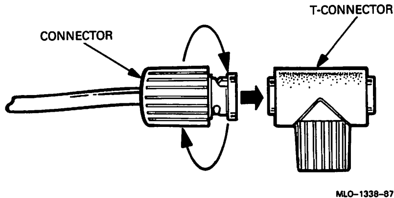
Figure 3-6: Connecting the T-connector to ThinWire
