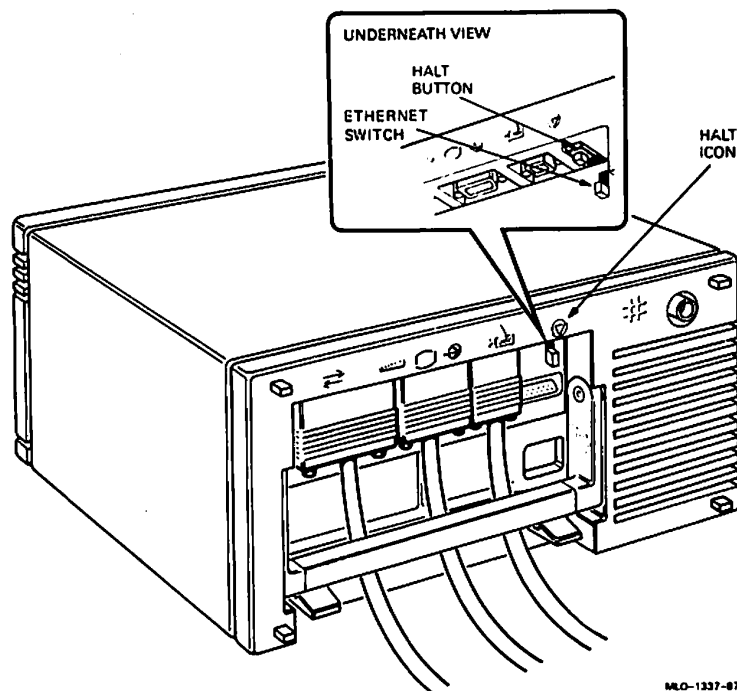
Figure 2-1: Setting the Switch for Standard Ethernet
