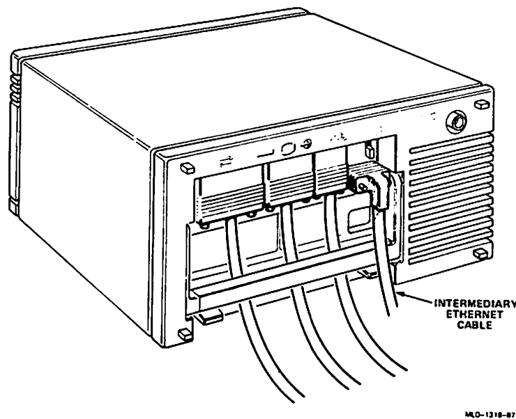
Figure 2-2: Connecting the Intermediary Cable
