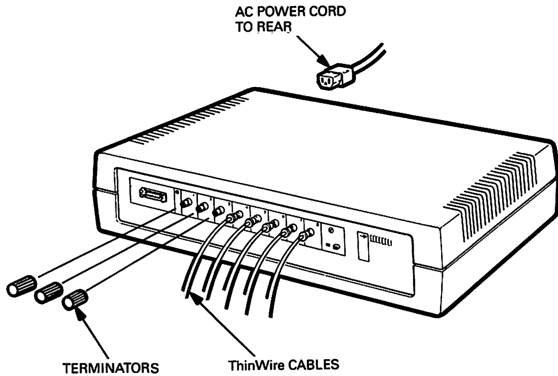
Figure 3-13: Terminator Connected to the DEMPR
