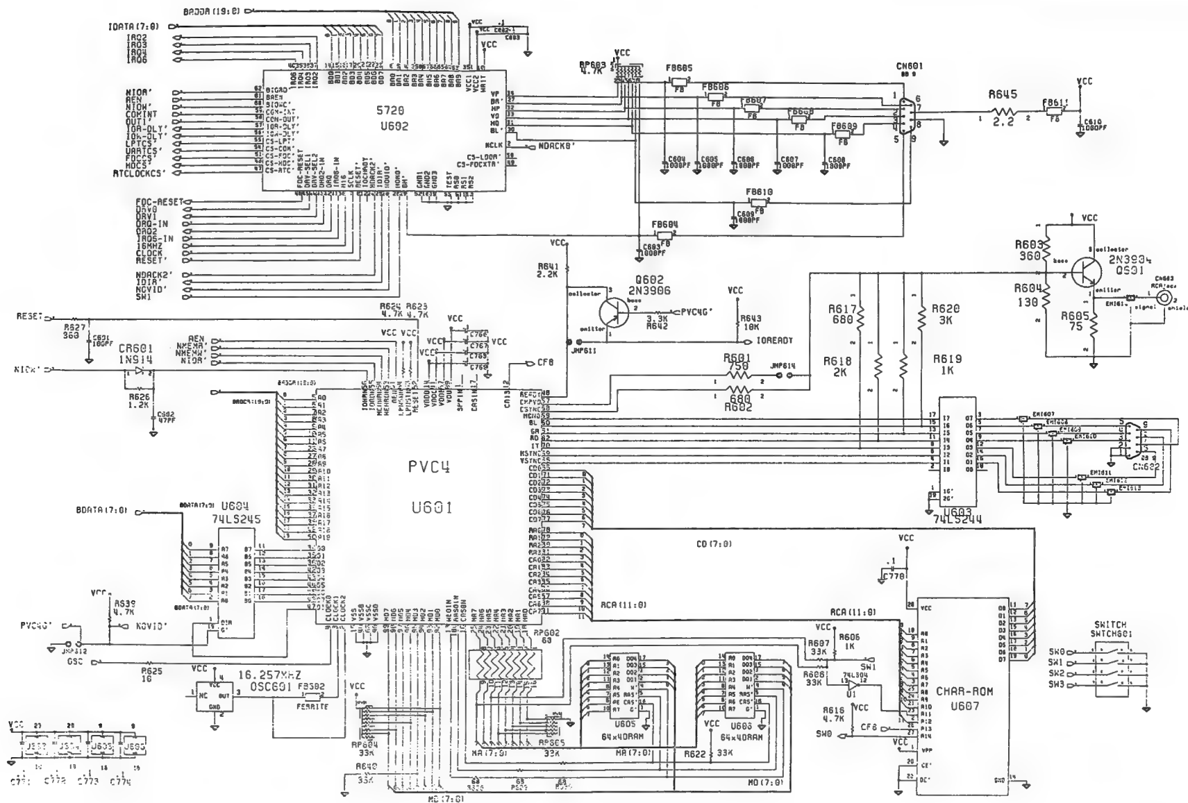
Schematic #312626 Sheet 6 of 6
