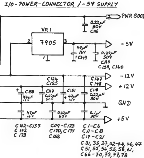
PCB ASSY. #380504 (sheet 8 of 8)
