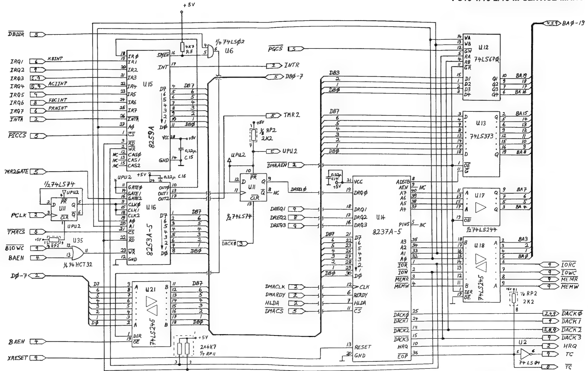
PCB ASSY. #380504 (sheet 2 of 8)
