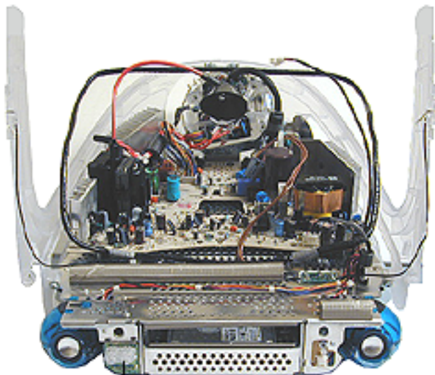
Headphone / Audio Board
