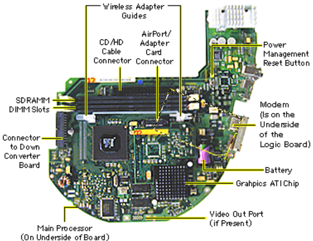
iMac 350 MHz Logic Board Diagram
