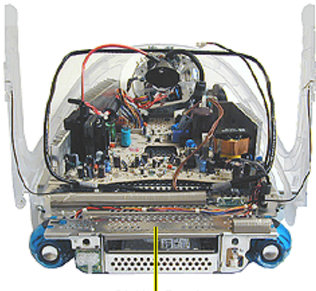
Divider Panel
