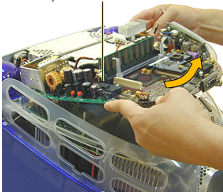
Logic Board/Down Converter
