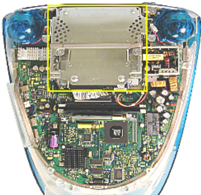
CD/HD Carrier
