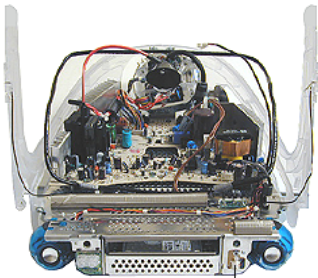
Power/LED Board
