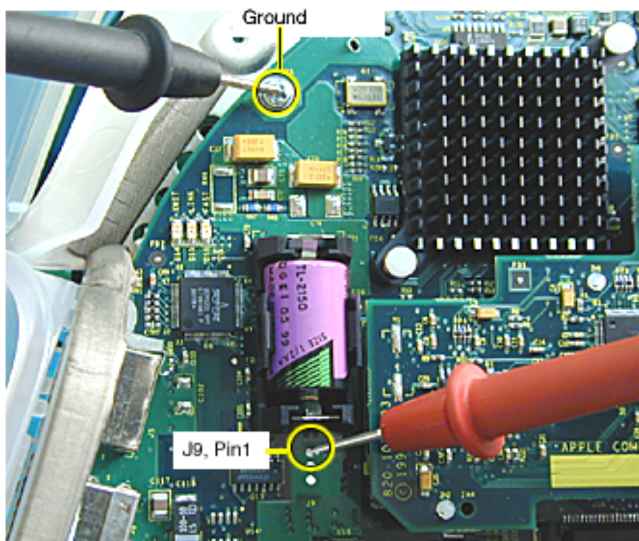
Testing for +5 V Trickle Power at J9 on the Logic Board
