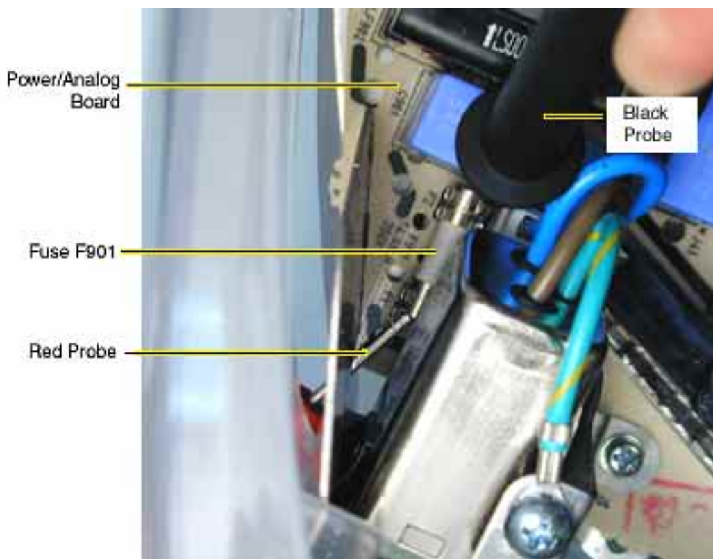
Testing Fuse 901 for Continuity
