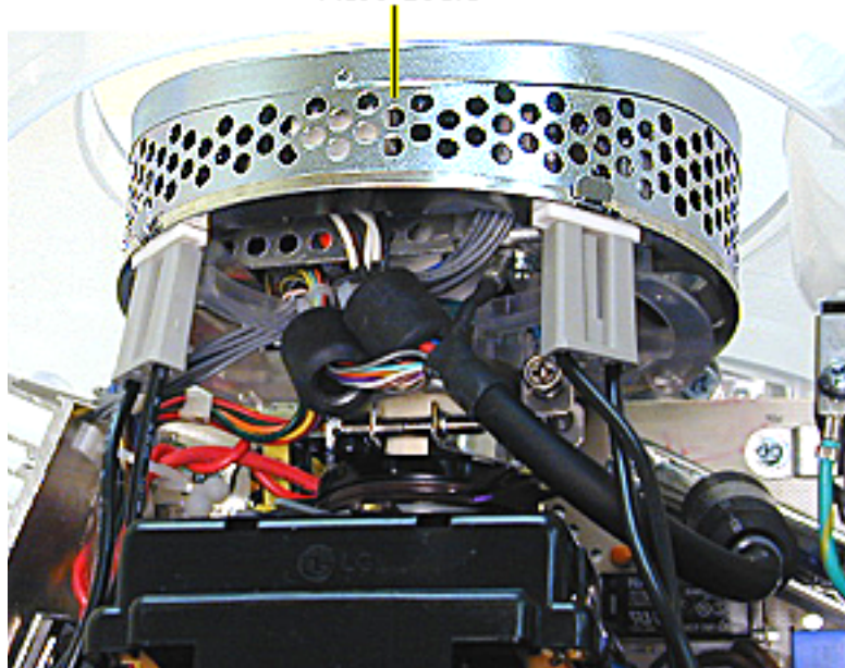
Video Board
