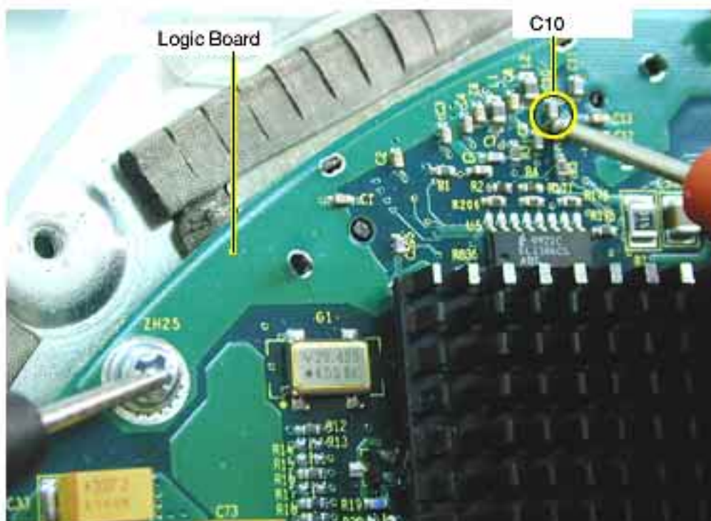
Testing DCO Voltages at C10 on the Logic Board
