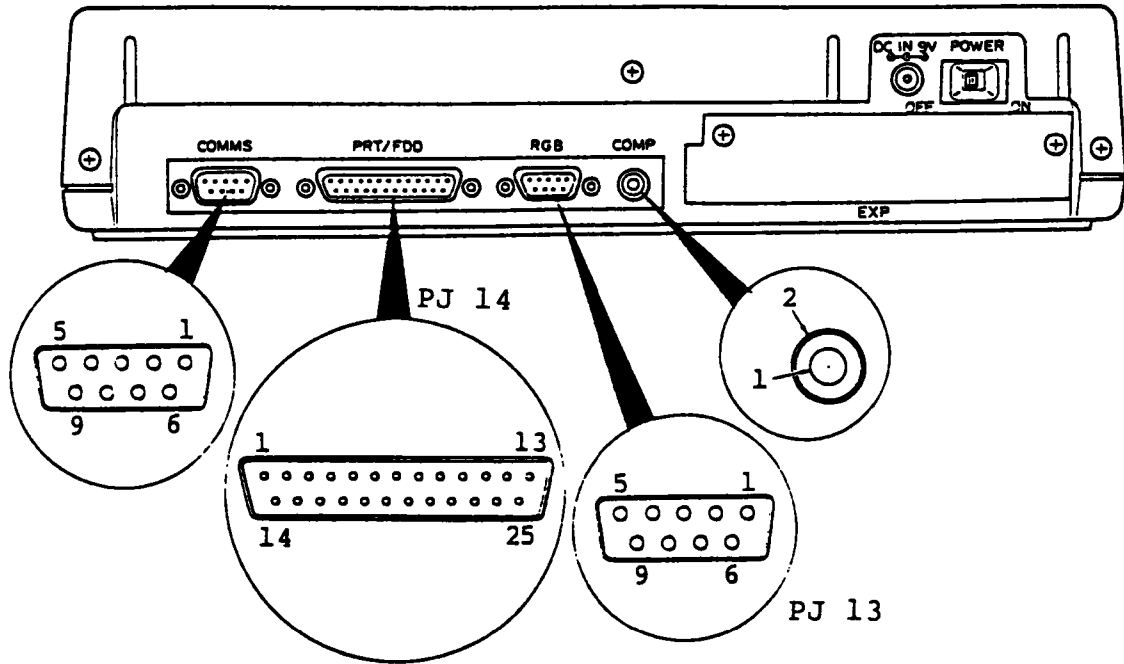
Figure 6-14 System Unit Rear Panel
