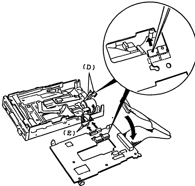
Figure 4-22 FDD PCB Removal
