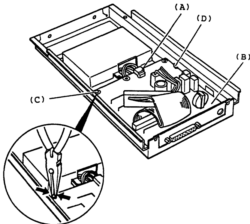
Figure 5-29 FDD PCB Removal
