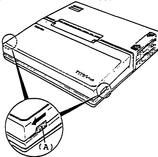
Figure 5-16 Opening the LCD
