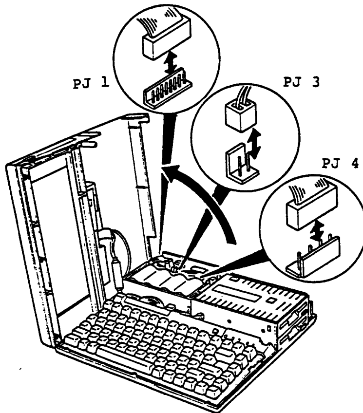
Figure 4-9 Connector Check
