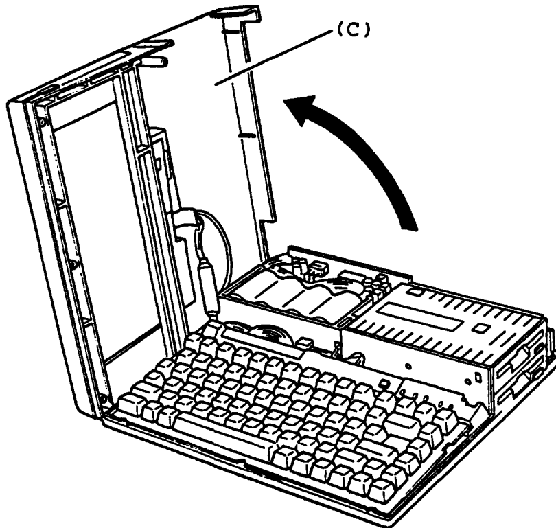
Figure 5-3 Disassemble the Upper Cover
