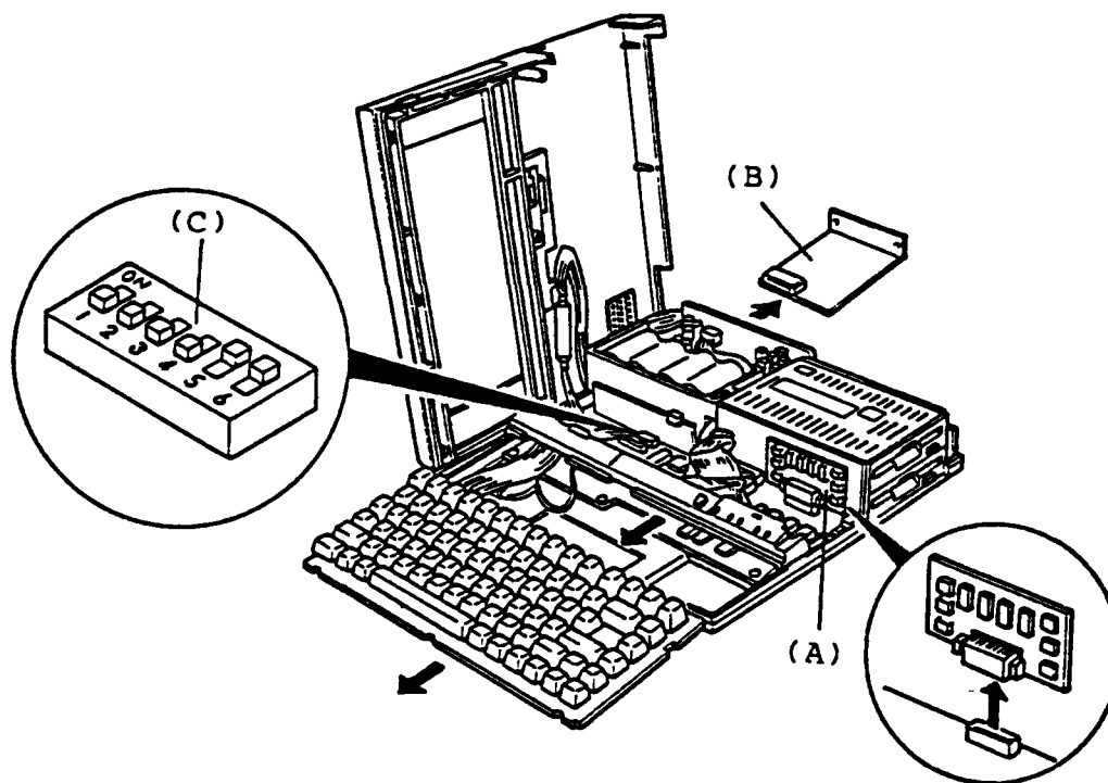
Figure 4-12 Option PCB Removal
