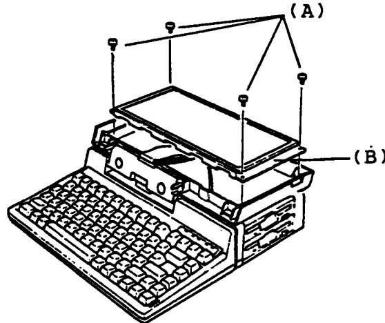
Figure 5-19 Four Screws Removal
