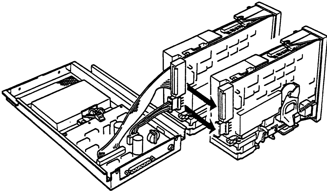
Figure 4-38 FDD Change
