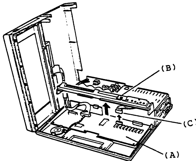
Figure 5-6 Indicator Plate Removal
