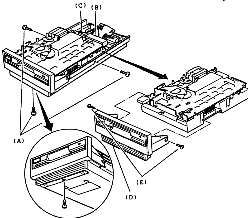
Figure 5-28 FDD Assembly Removal
