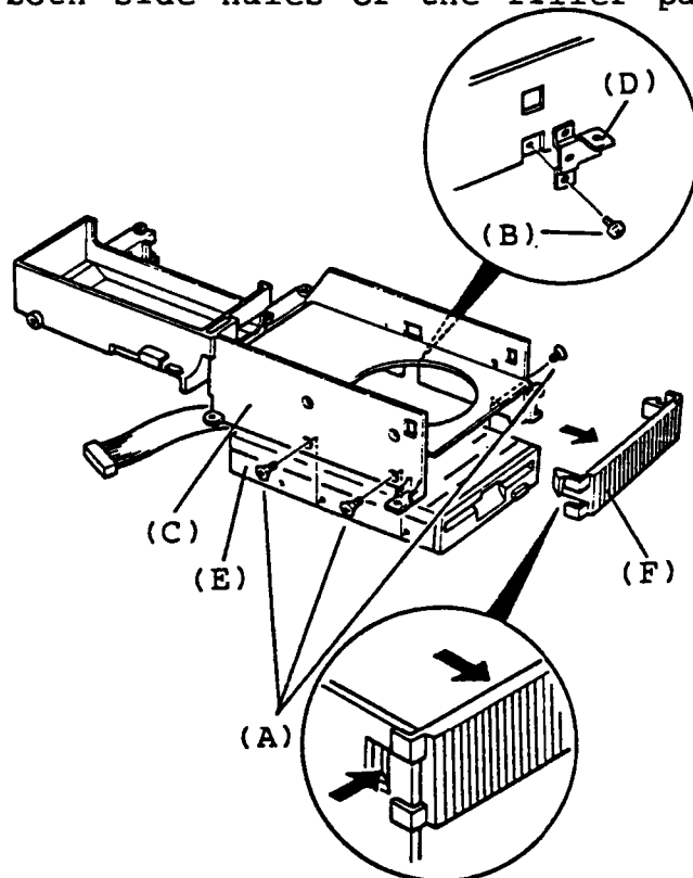
Figure 5-10 Floppy Disk Drive Removal (F type)
