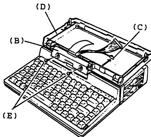
Figure 5-21 Peeling the Seal
