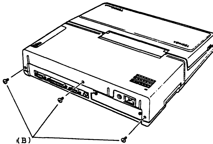
Figure 5-2 Three Screws removal
