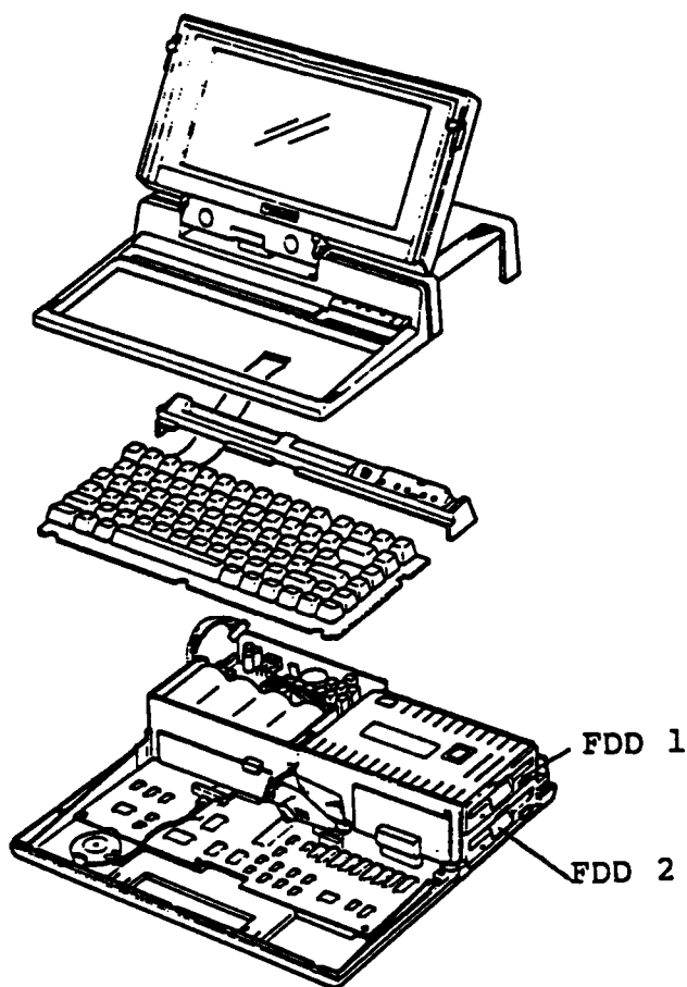
Figure 4-15 T1100 PLUS System Unit (F/F type)
