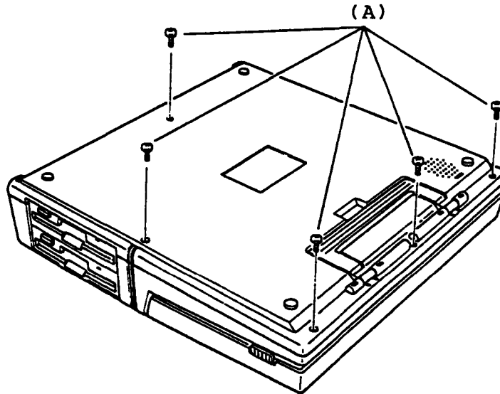
Figure 5-1 Five Screws Removal
