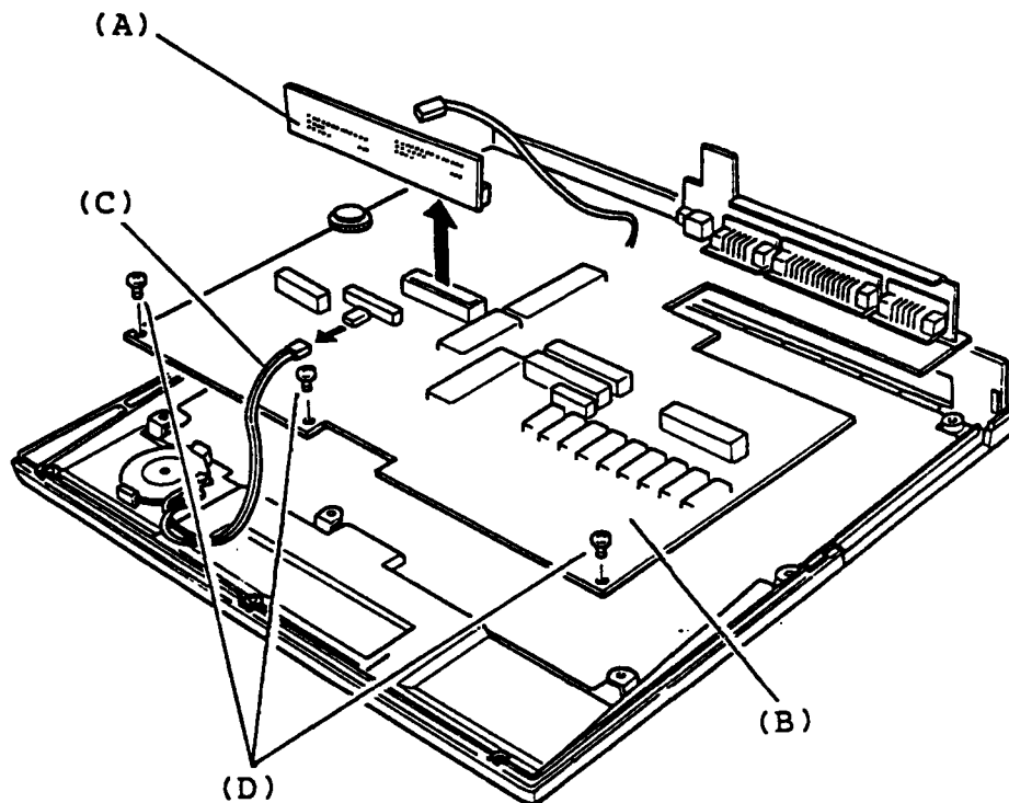
Figure 5-14 System PCB Removal
