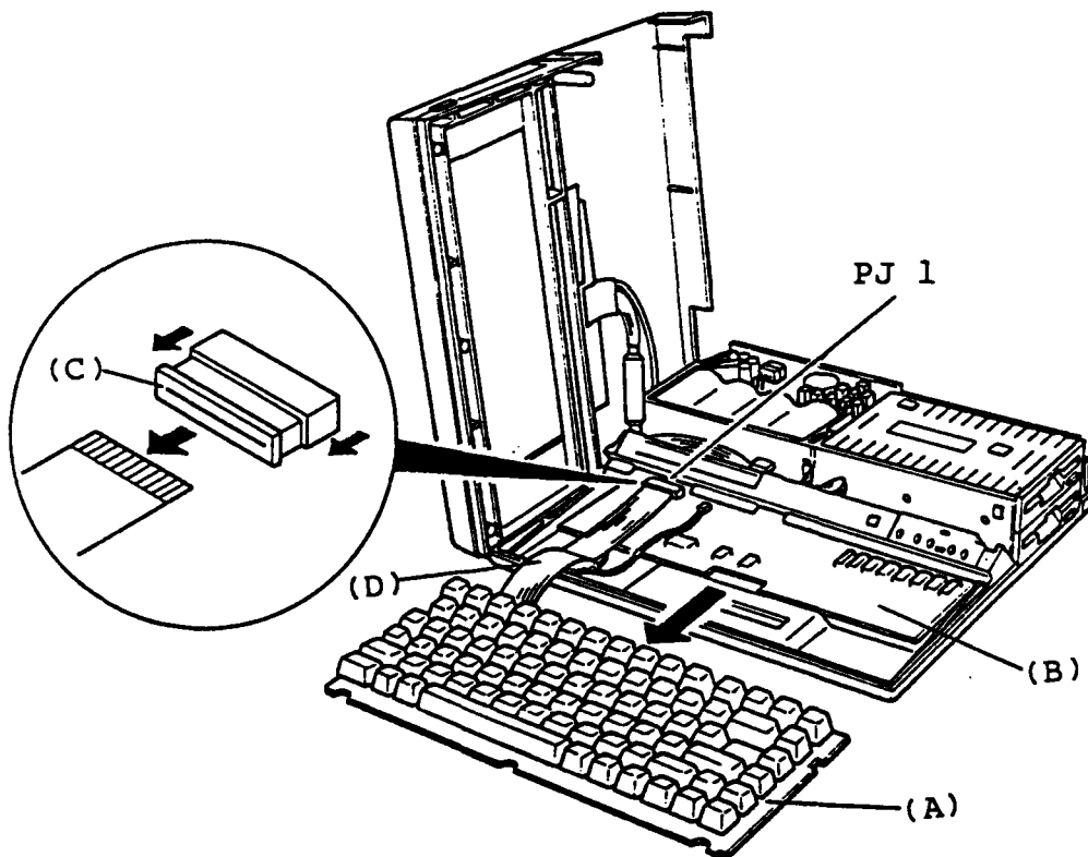
Figure 5-5 Keyboard Unit Removal
