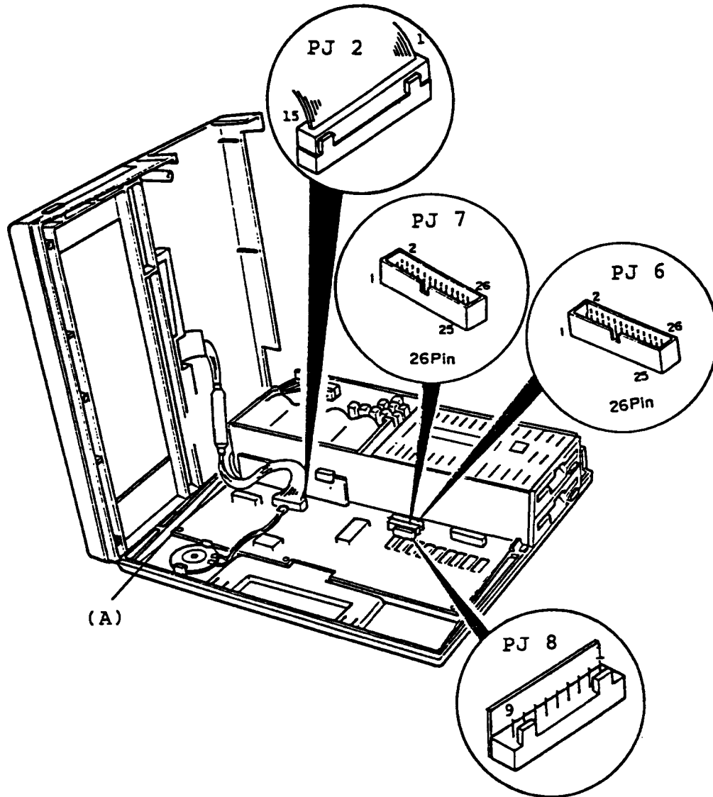
Figure 4-14 Voltage Check
