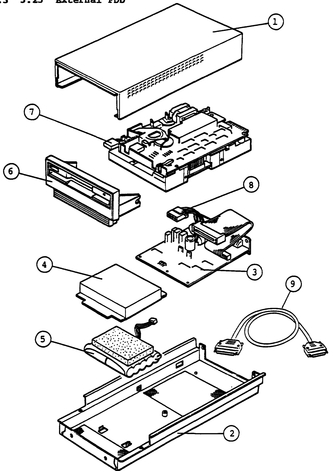
Figure 7-3 5.25" External FDD
