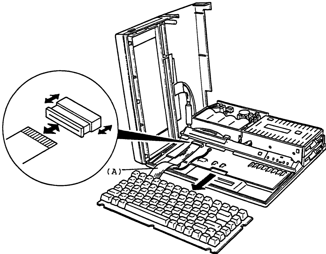
Figure 4-25 Connector check
