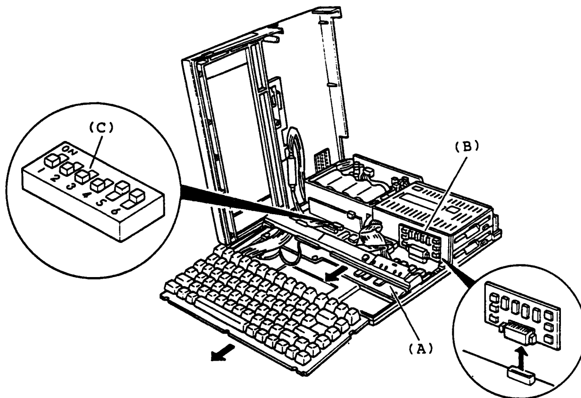
Figure 5-24 Memory Card Removal
