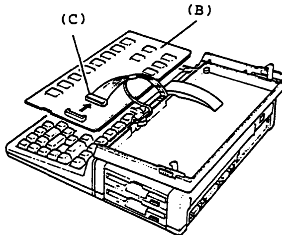
Figure 5-20 LCD Removal
