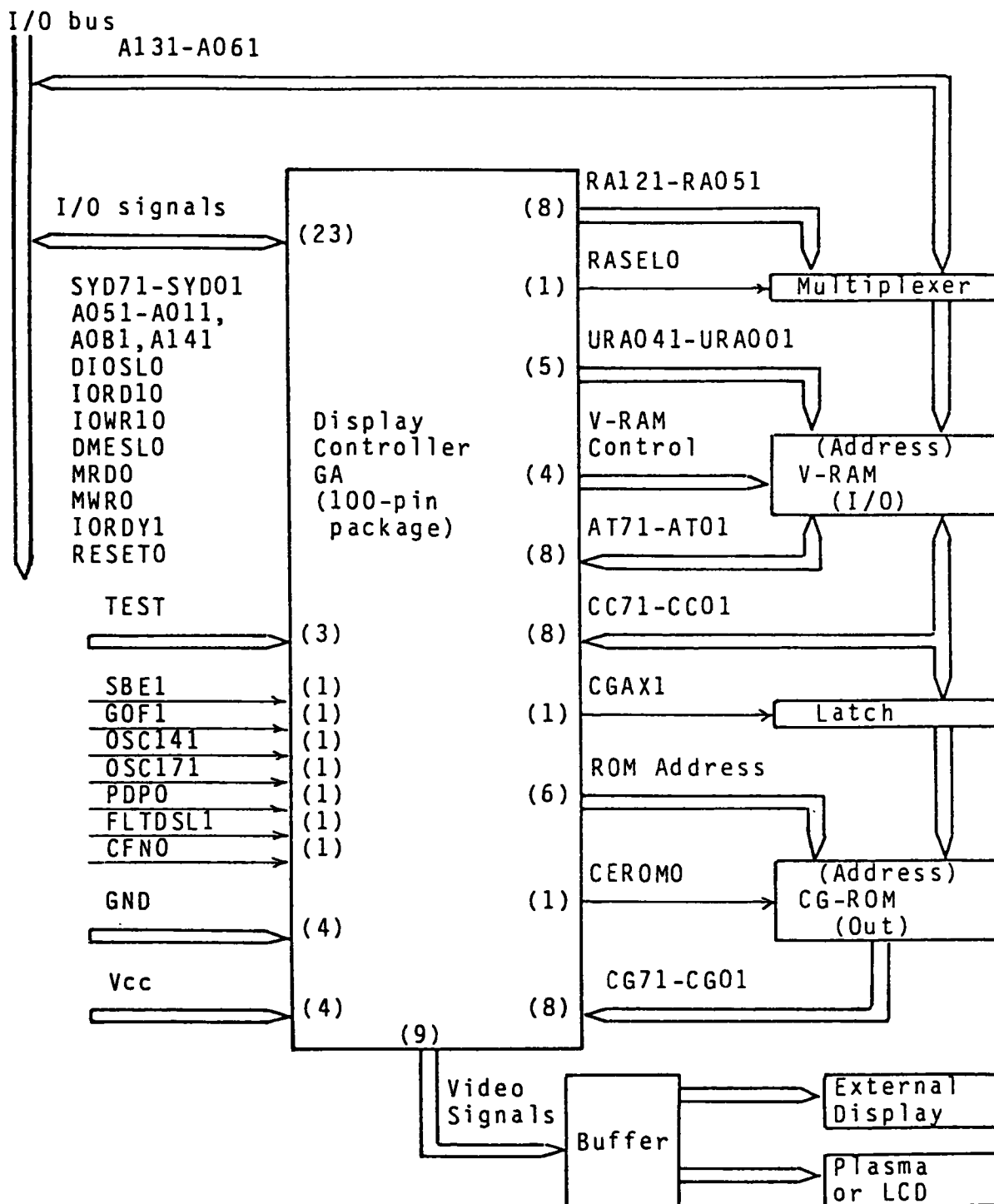
Figure C-1 Display Controller Subsystem (DCS)
