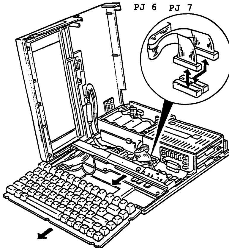
Figure 4-18 Connector Check
