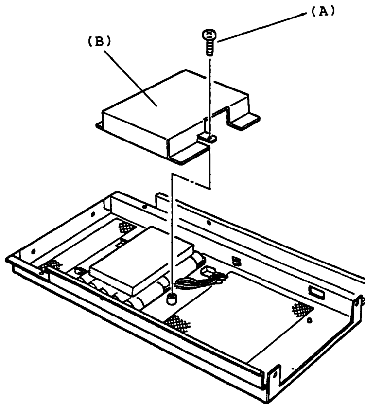
Figure 5-30 Battery Removal
