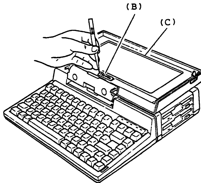
Figure 5-17 Peeling the Seal
