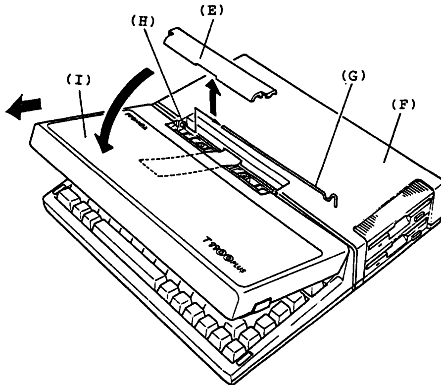
Figure 5-23 LCD Rear Cover Removal
