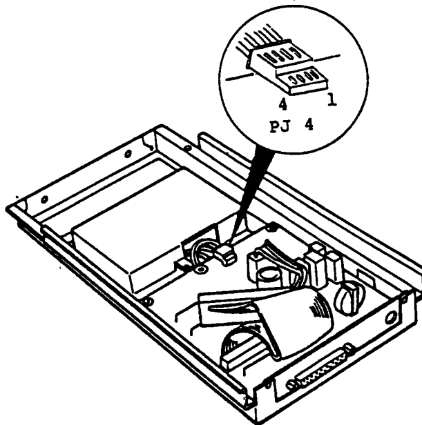
Figure 4-35 Voltage Check
