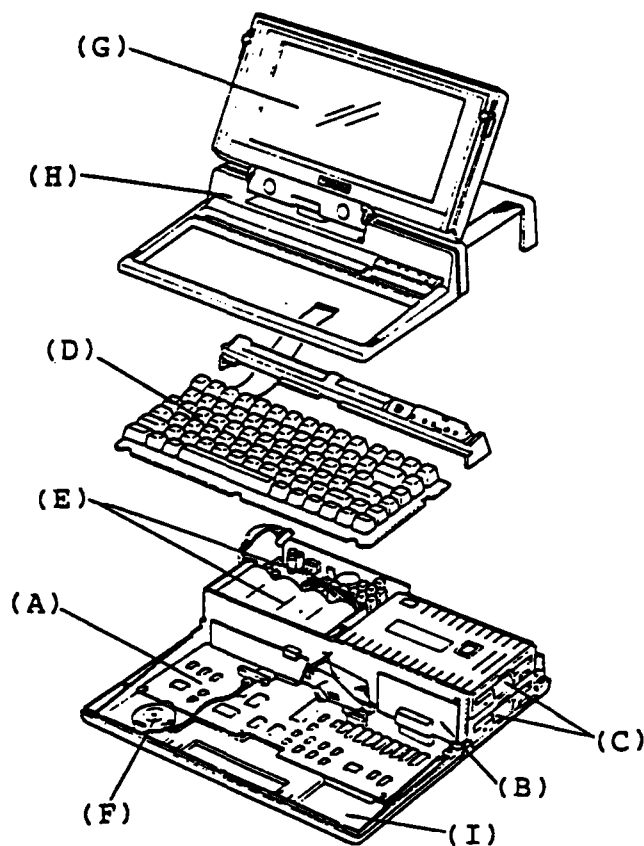
Figure 6-1 Front View of System Unit
