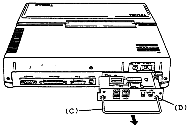
Figure 5-26 Modem Card or I/O Expansion Card Removal
