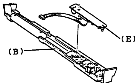
Figure 5-7 Indicator Removal
