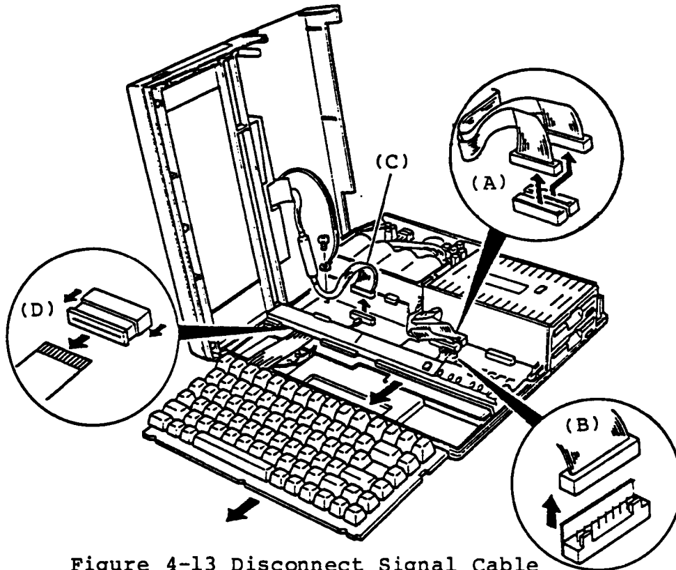
Figure 4-13 Disconnect Signal Cable
